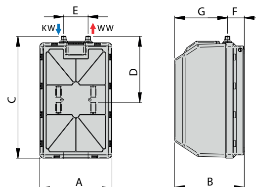
Undersink version 10-15
