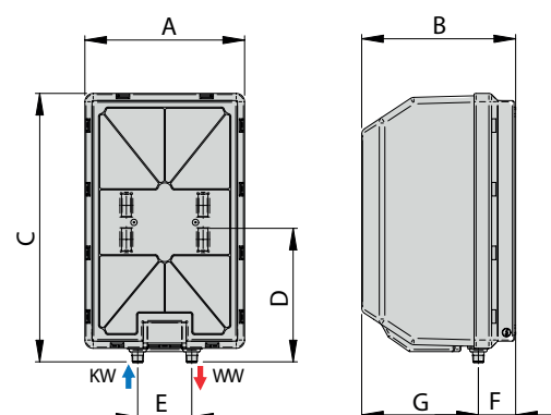
Oversink version 10-15-30
