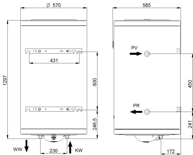
Fig./Abb. 9 - VERTICALI TERMO SOLARI/ VERTICAL SOLAR THERMO- ELECTRIC / VERTICALES TERMO SOLAR/ VERTICAIS TERMO SOLAR (200 )
