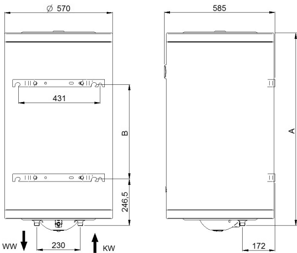
Fig./Abb. 8 - VERTICALI / VERTICAL / VERTICALES / VERTICAIS ( 150 – 200 )
